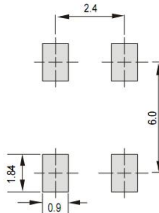
Mounting PAD Layout(mm)
